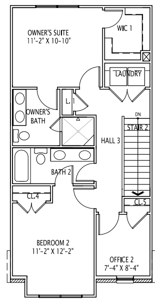
THIRD FLOOR PLAN
