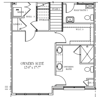
THIRD FLOOR PLAN - OPTIONAL FRONT OWNER'S SUITE (REPLACES LIVING ROOM & DINING ROOM)
