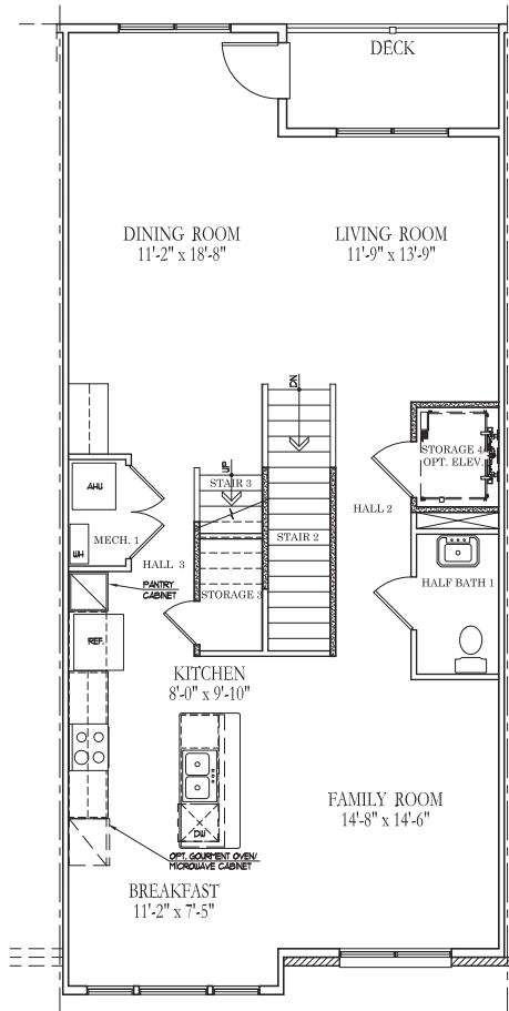
ALT. 1 THIRD FLOOR PLAN
