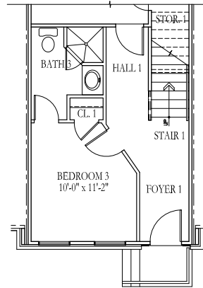
ALT. FIRST FLOOR PLAN W/ OPT. BEDROOM & FULL BATH 3
