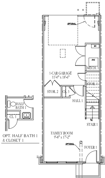
ALT. FIRST FLOOR PLAN
