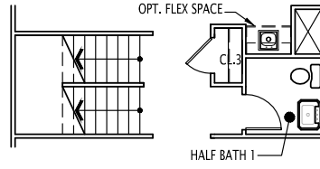
SECOND FLOOR - OPTIONAL CLOSET
