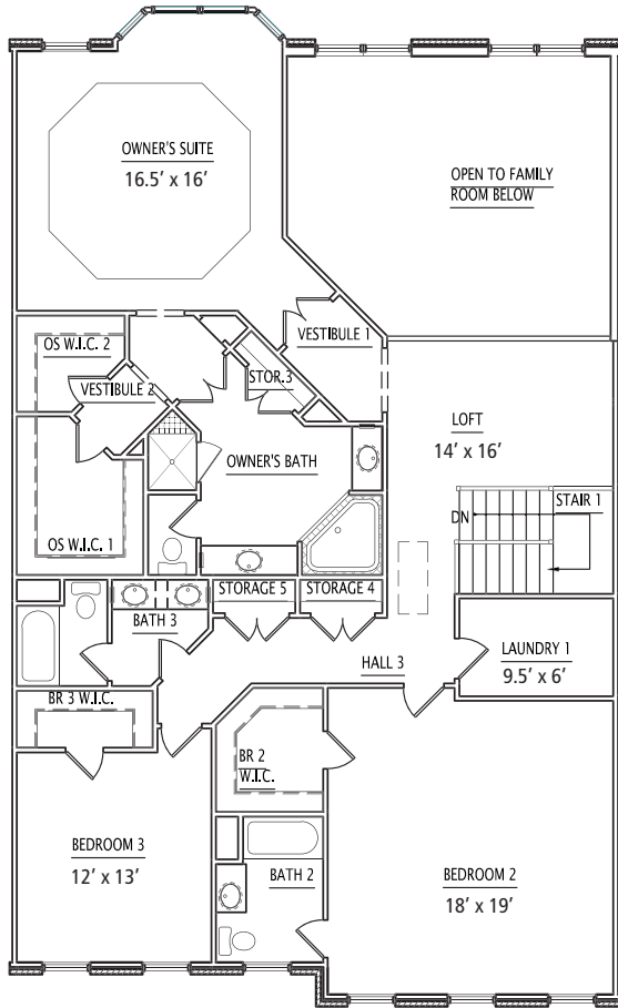
A Alternate Second Floor Ceilings: 9'
