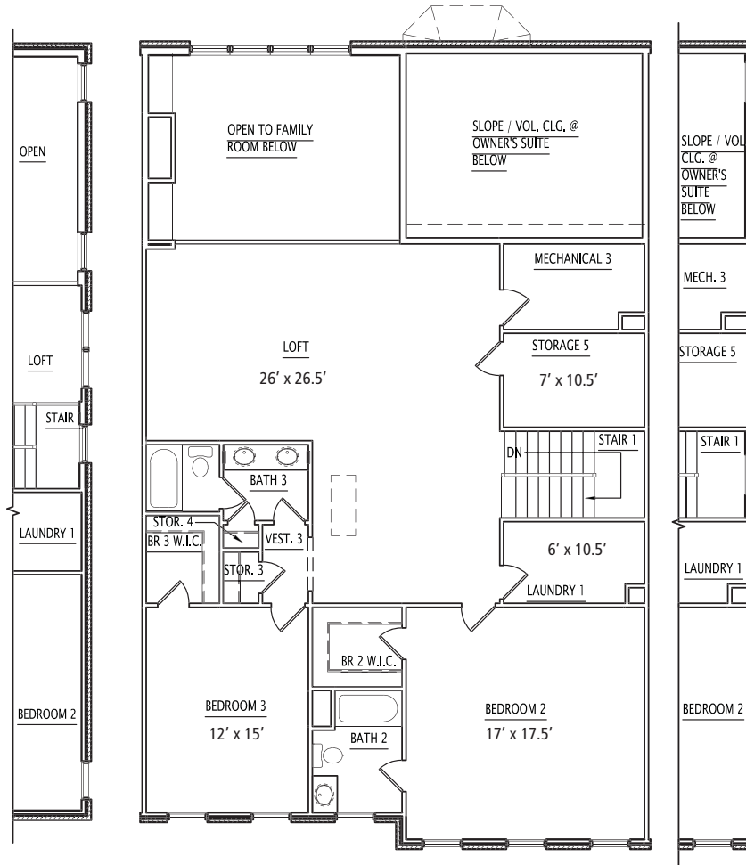
B Alternate Second Floor Ceilings: 9'
