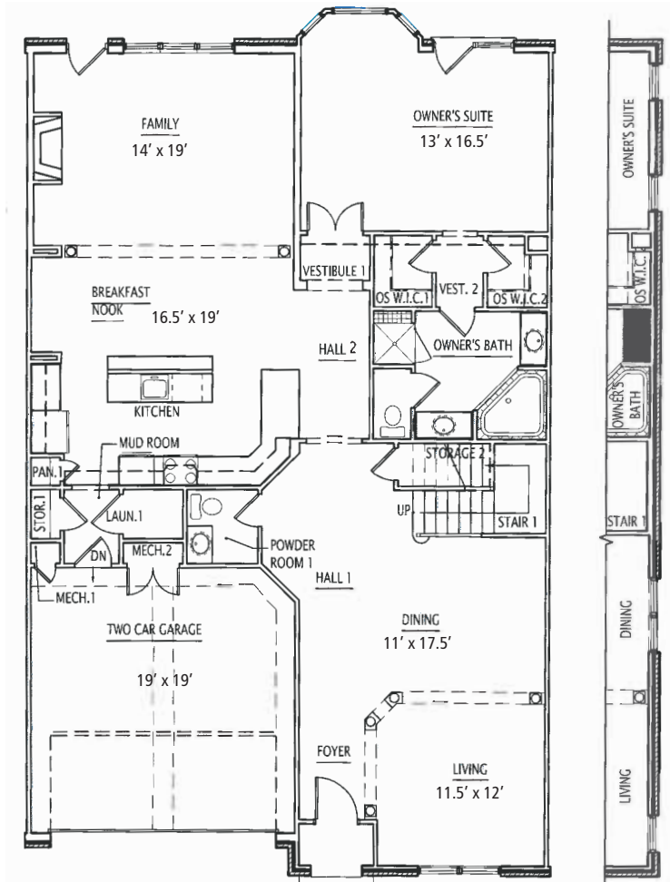
1 ST GROUND FLOOR Ceilings: 10'
